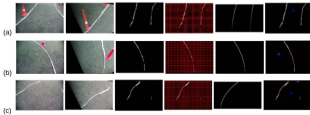
Fig. 5. From left to right (1) Acquired image from the camera (2) Top view image (3) Preprocessed image (4) Clustered image (5) Estimated lane model (6) Estimated heading point. The results clearly demonstrate that objects and white patches appearing close to the lanes do not have any adverse effect on the performance of the algorithm.
