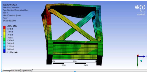
Fig. 2. Structure with Cross-Member
